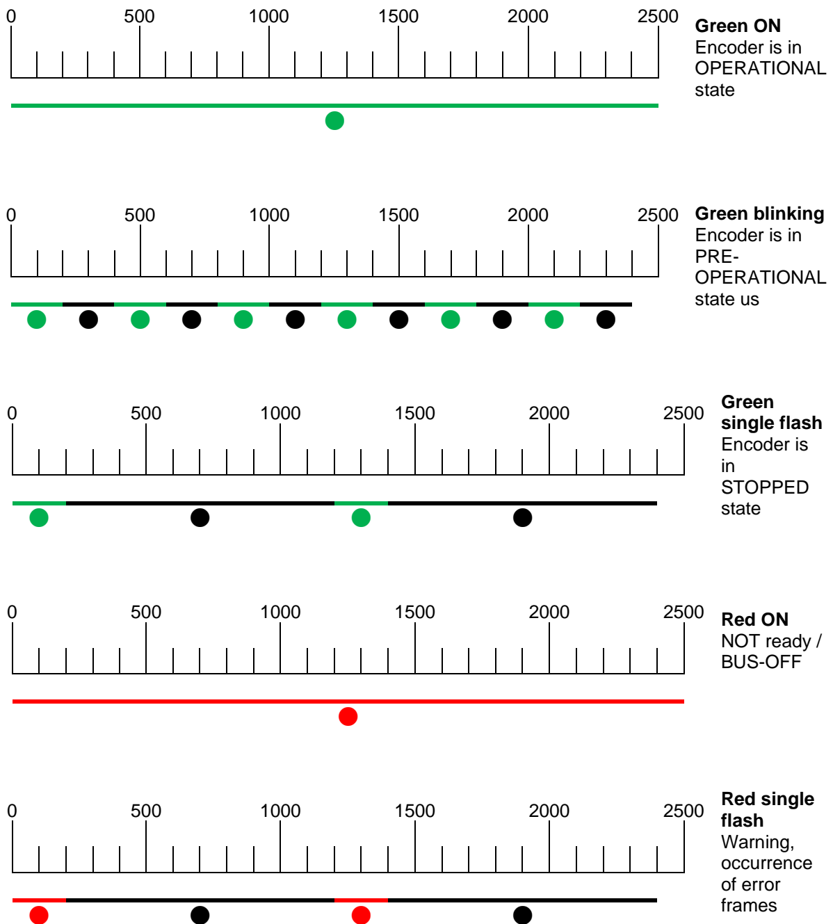
Figure 3.2: LED indications 1
